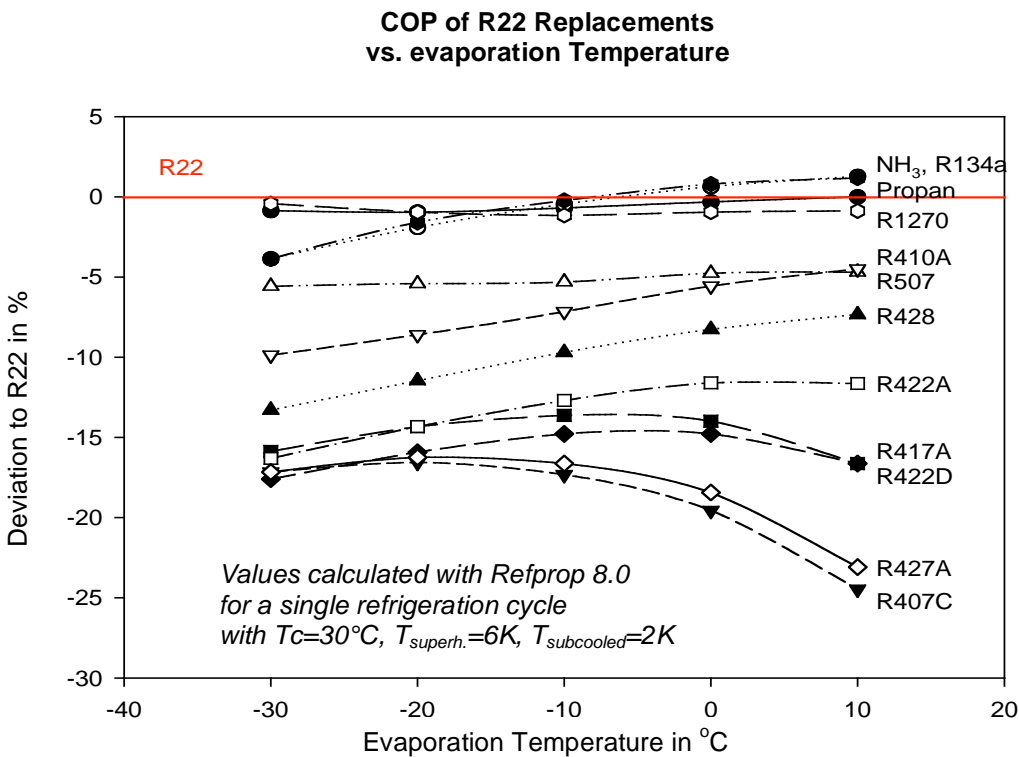
Fig. 2: COP comparison of different R22 substitutes
